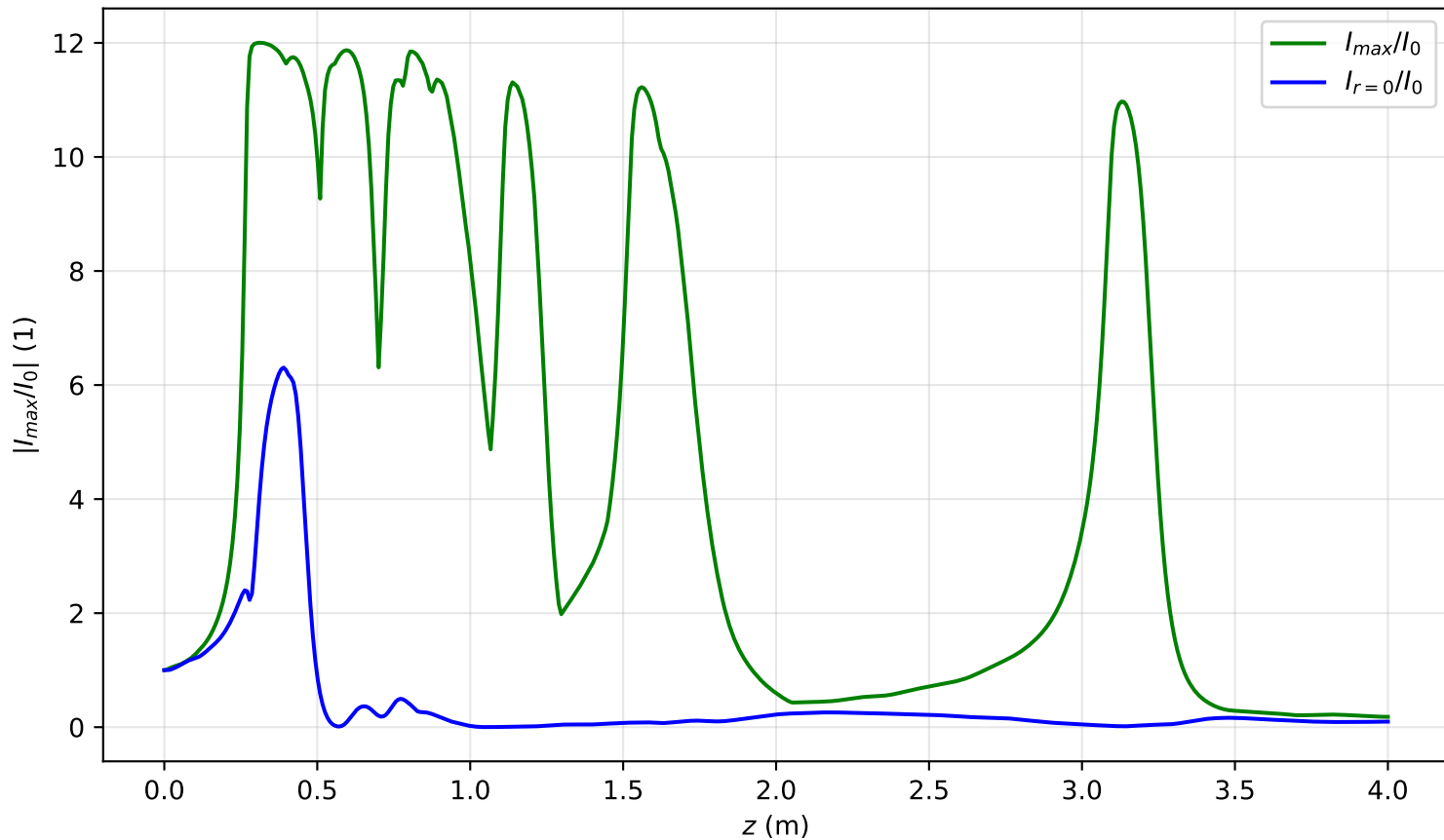
I_{max}(x = 0, y = 0, z)/I_0 , Pin=9.2Pcr, noisy input, artificial time
